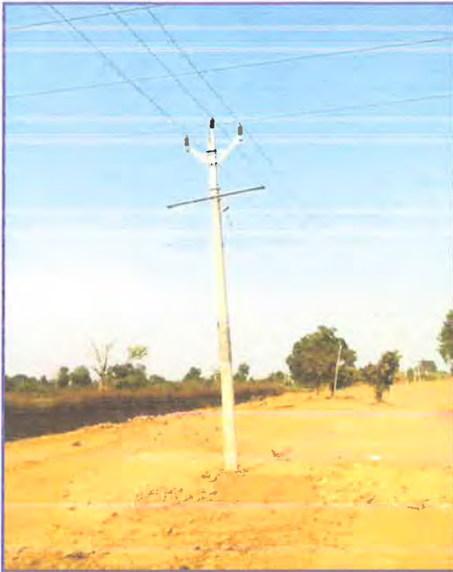
HT Line work in progress at Kanchanpur & Saliya phatak Village 33KV Islamnabad to Pan Umaria Feeder Katni District
