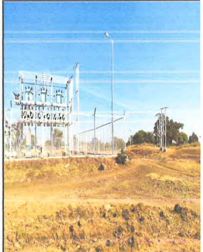
Cable Trench Line & Fencing Work at 33/11KV BIJURI S/s District Chhindwara
