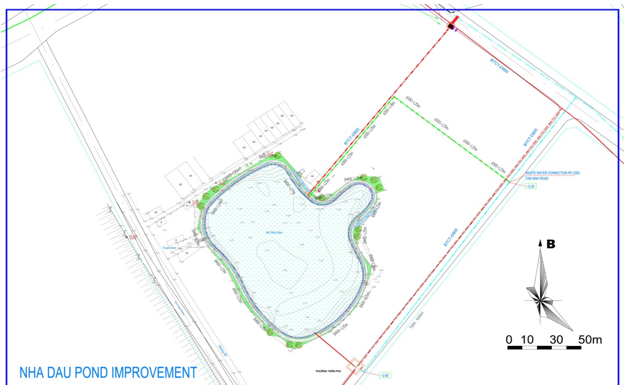
Figure 4. Improvements to the collection and separation of WW and stormwater
