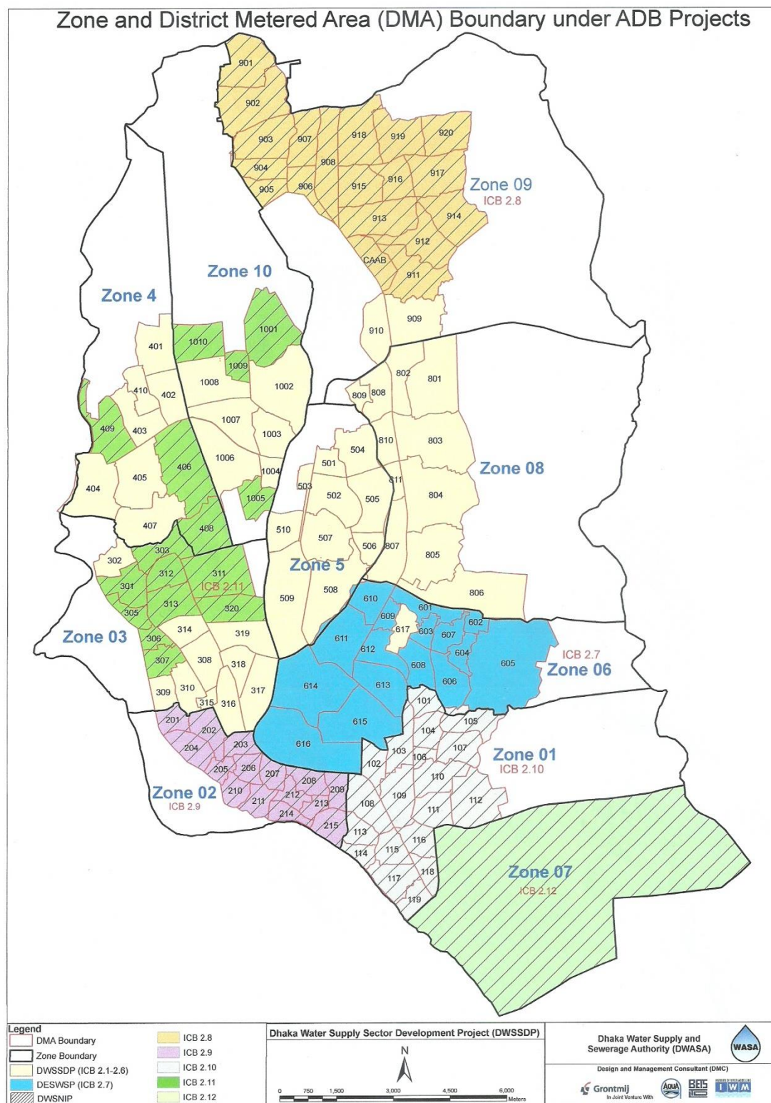
Figure 2: DMA Map Showing Locations of DMAs covered in Package No. ICB 2.9
