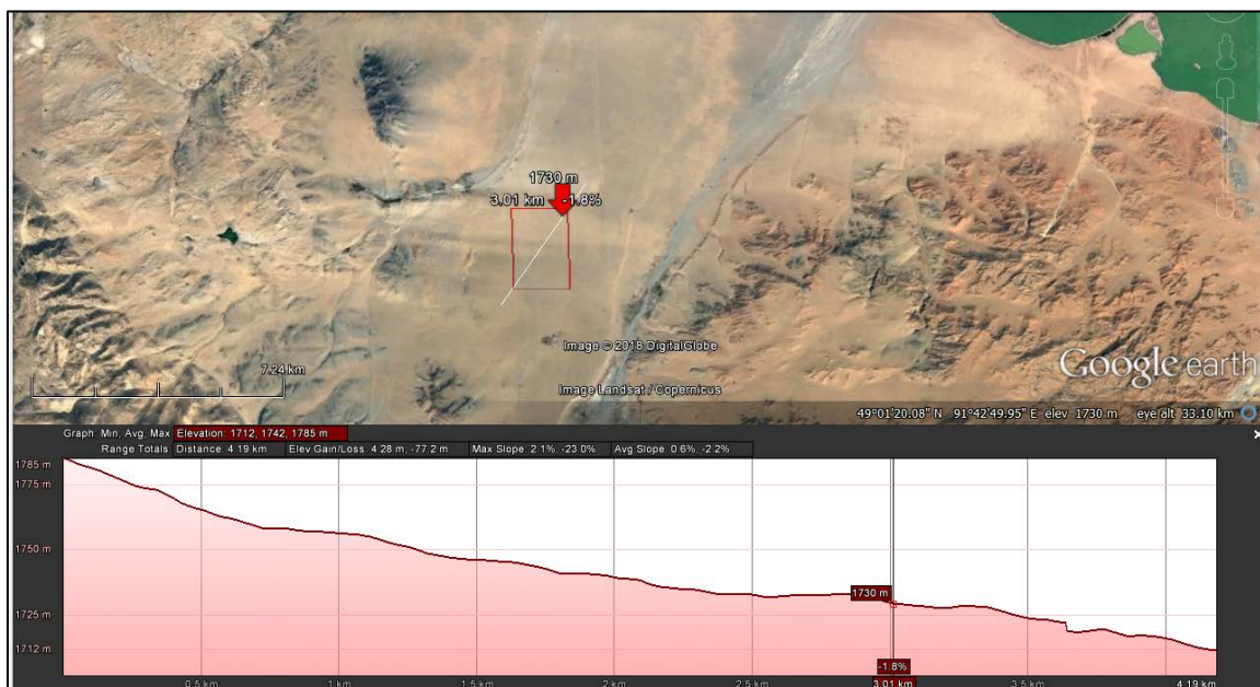
Figure 35: Umnugovi wind farm site topographical profile.
