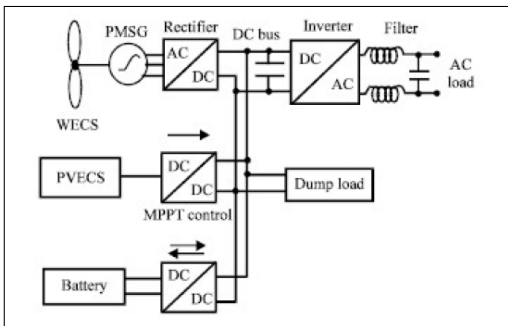
Figure 23: Conceptual design, Altai Soum hybrid RE system.
