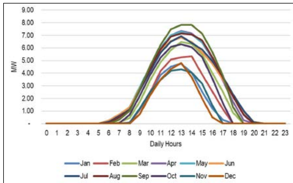
Figure 60: Govi-Altai solar PV daily profiles by season (MW).
