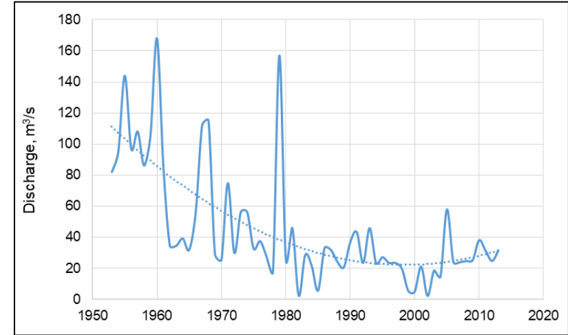
Figure 53: Trend of annual maximum discharge, Chigestei River.
