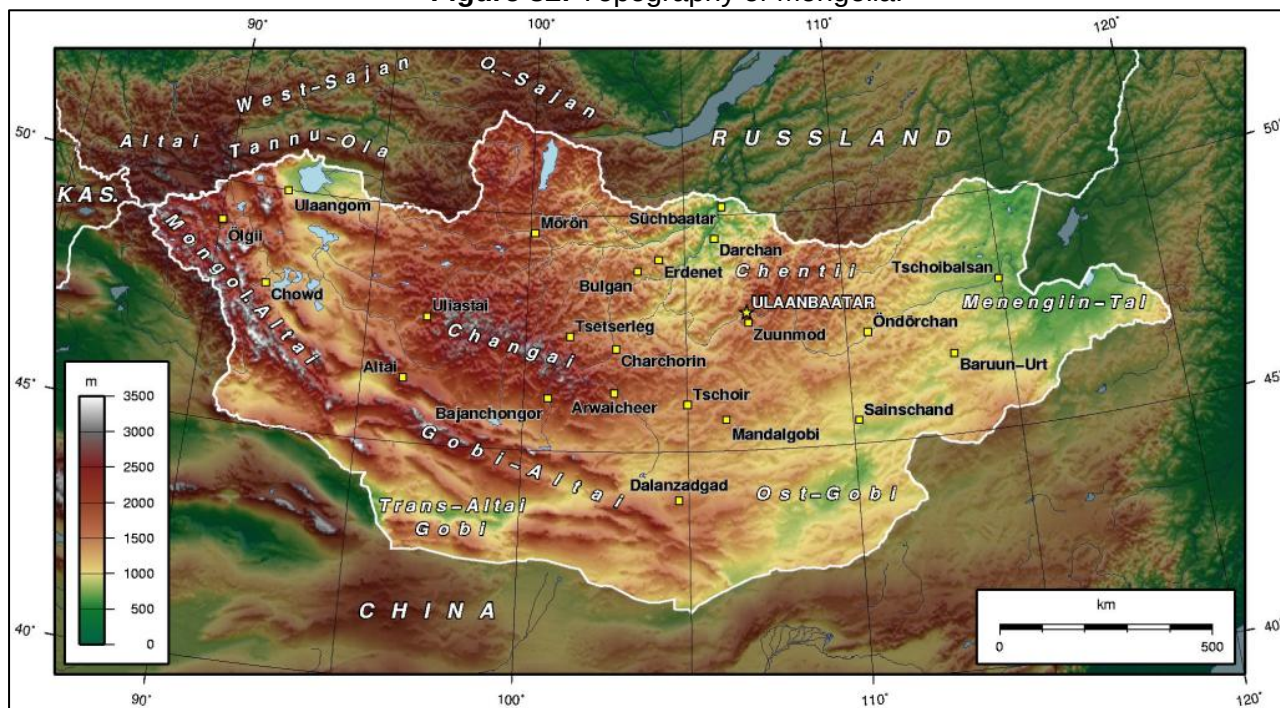
Figure 32: Topography of Mongolia.
