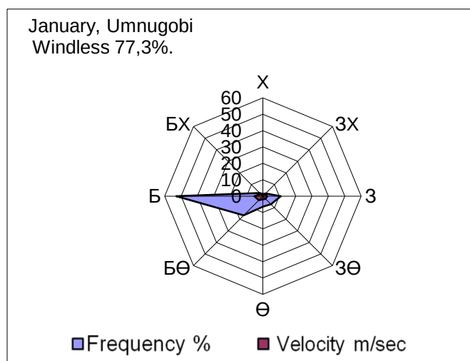
Figure 40: Umnugovi wind roses.
