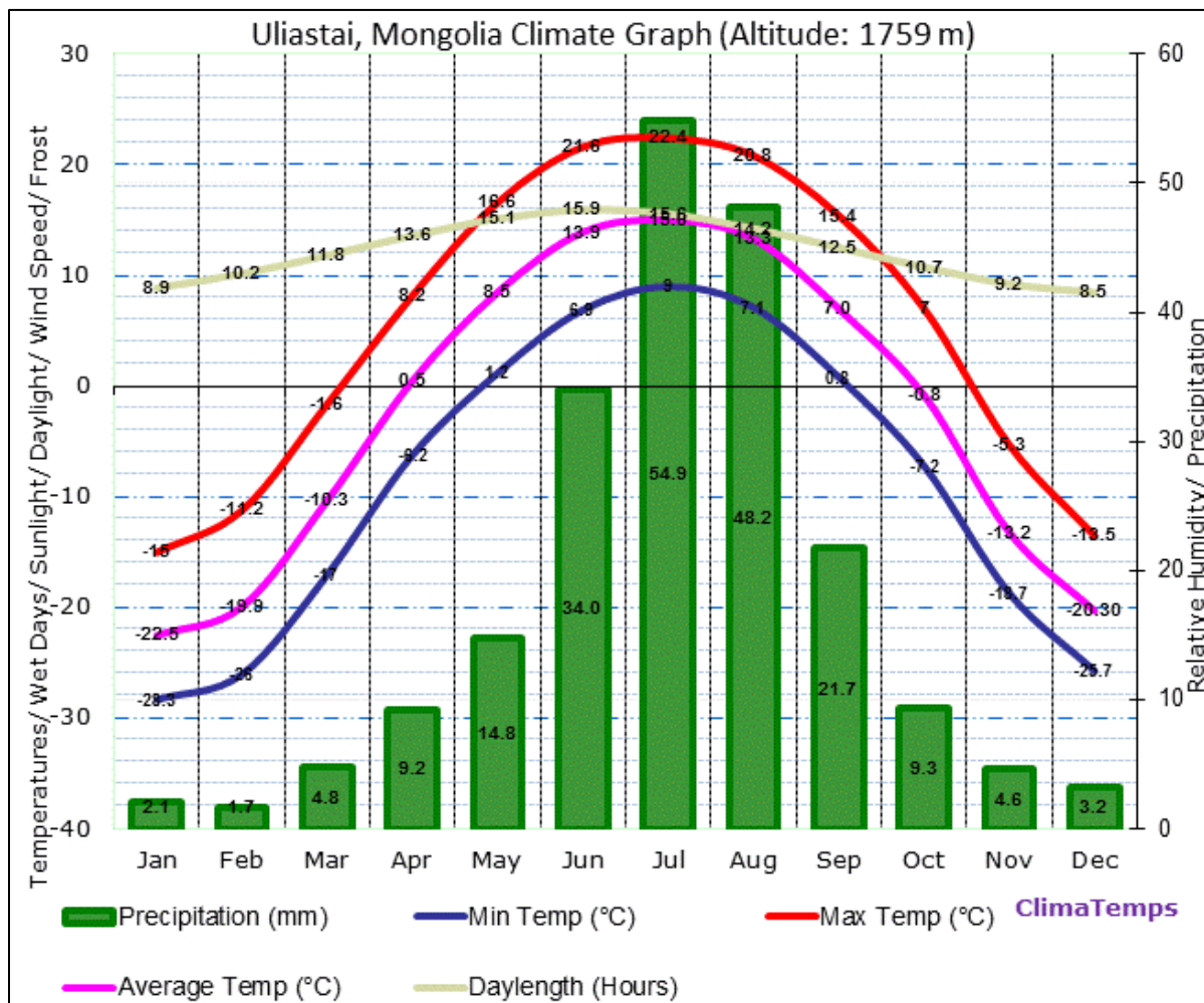
Figure 49: Uliastai City climatogram.
