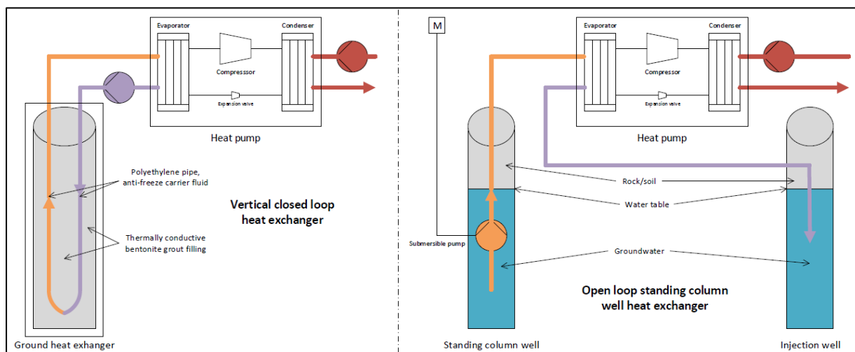
Figure 83: Closed and open loop heat exchangers.
