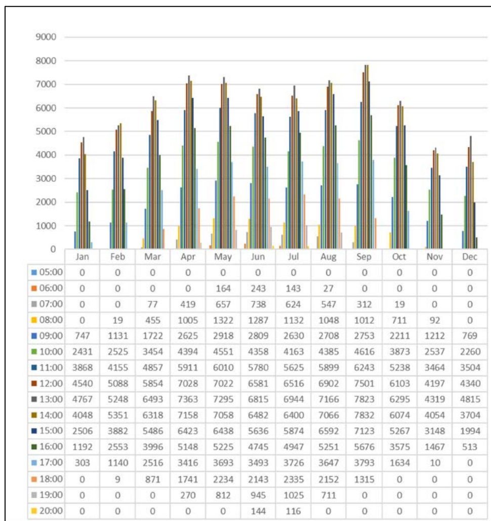
Figure 18: Govi Altai solar PV farm estimated production (kWh/hr).
