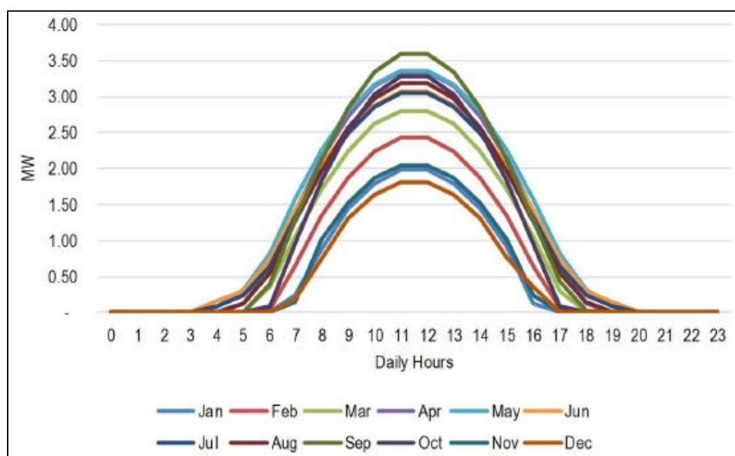
Figure 50: Uliastai Solar PV Daily Profiles by Season (MW).
