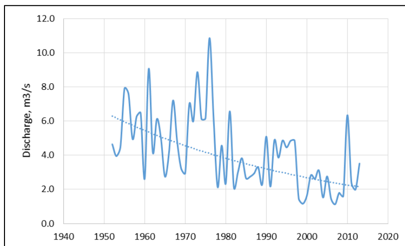
Figure 52: Trend of annual mean discharge, Chigestei River.
