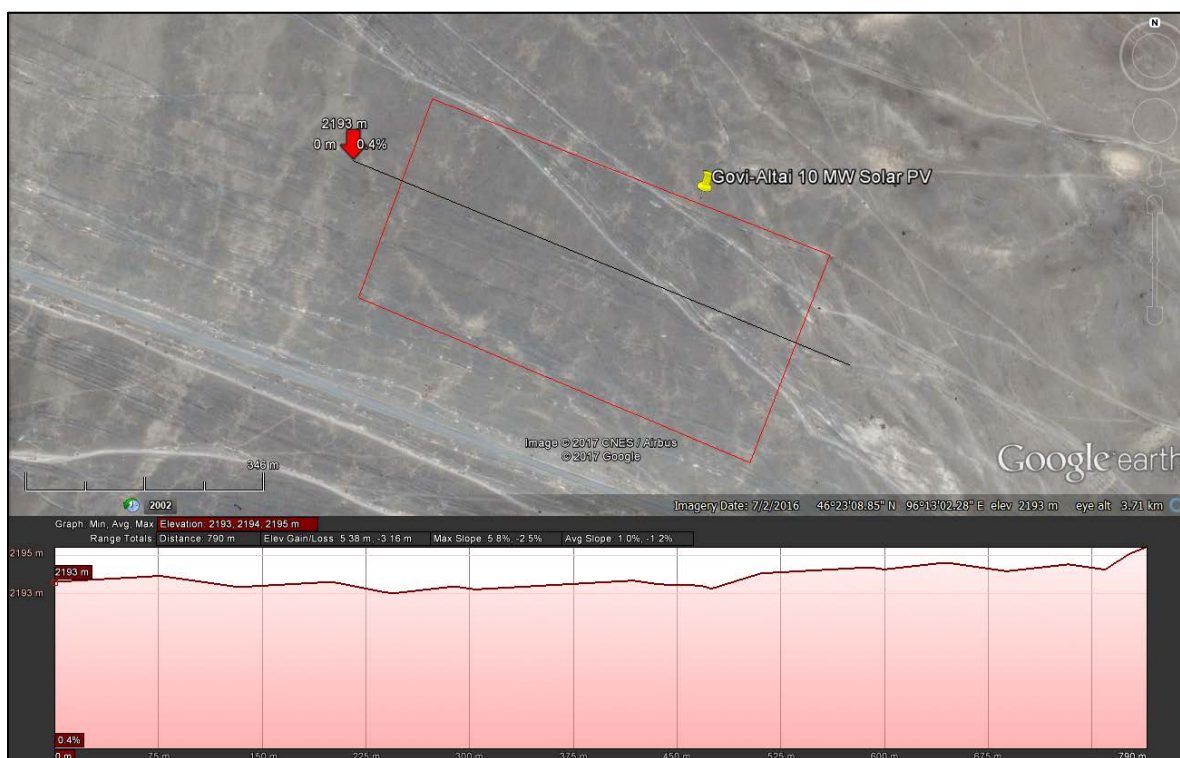
Figure 56: Govi Altai Solar PV site topographical profile.
