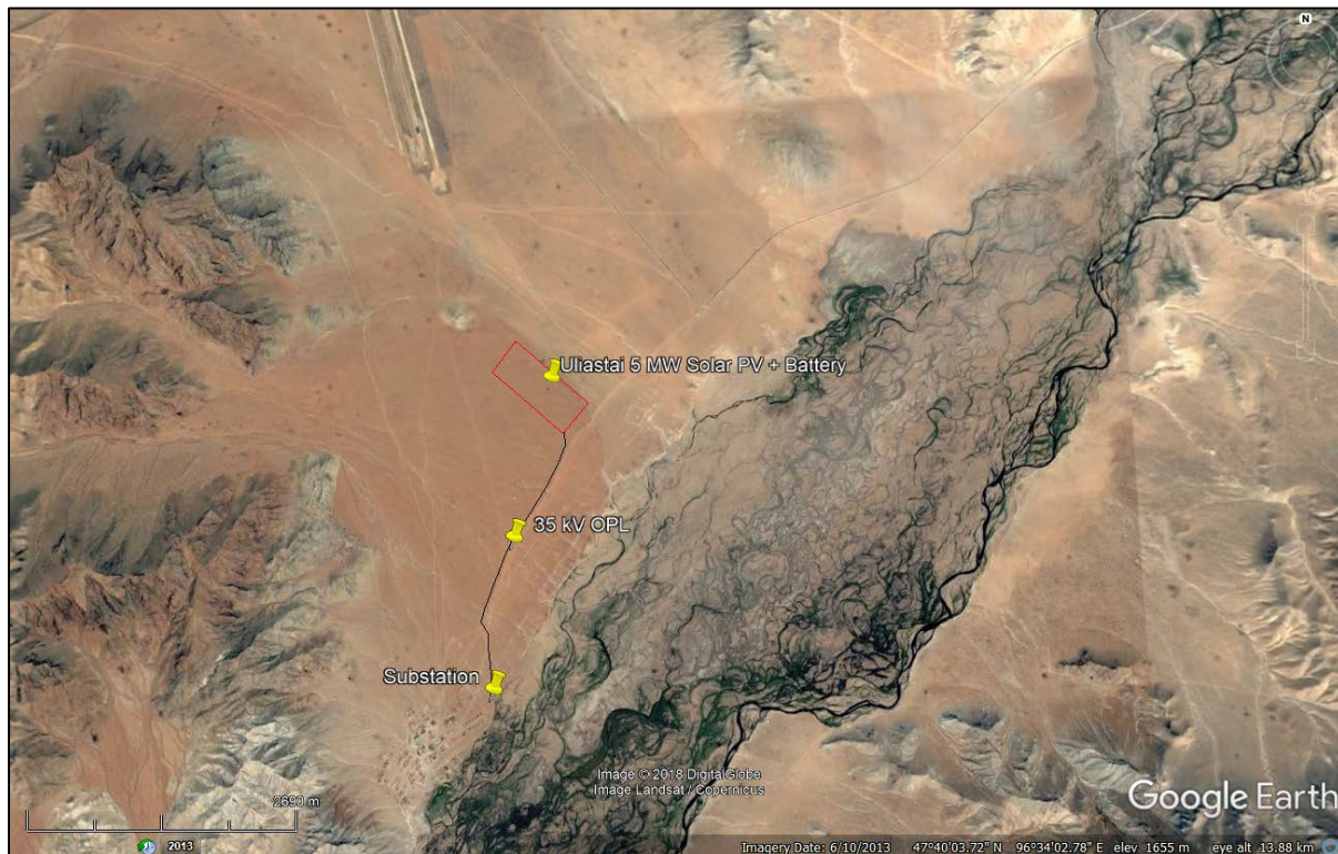
Figure 7: Solar PV farm location, Mandaat Bag, Aldarkhaan Soum, Zavkhan Aimag. OPL location is indicative.
