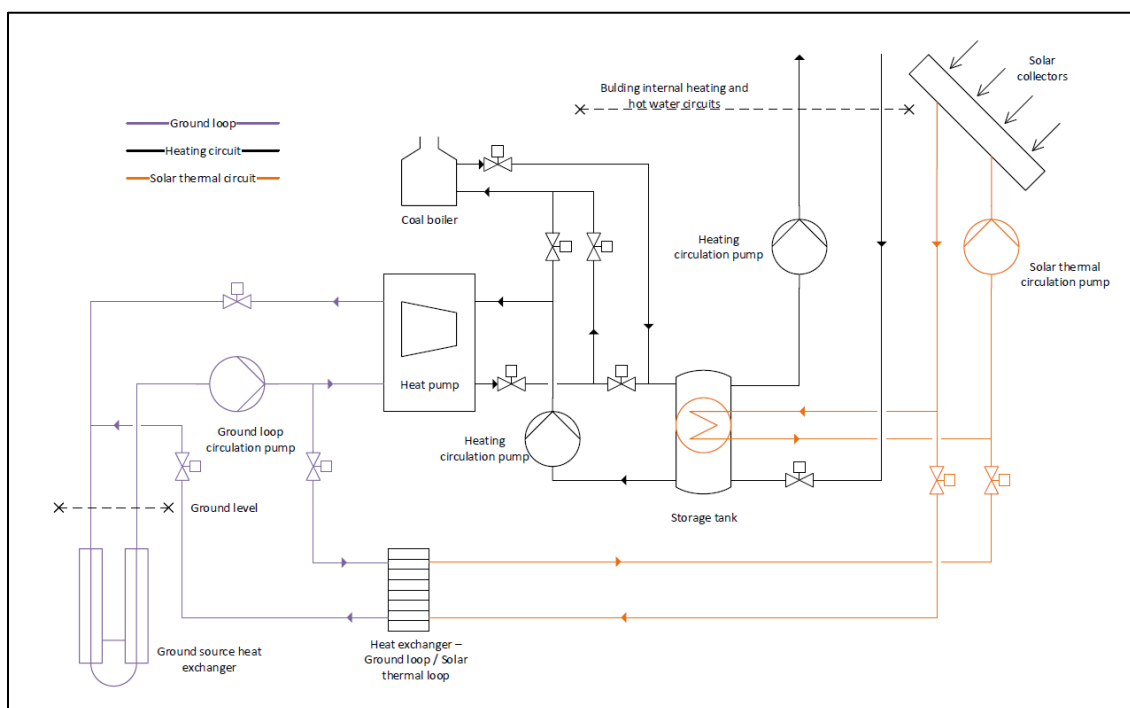
Figure 31: GSHP system schematic.
