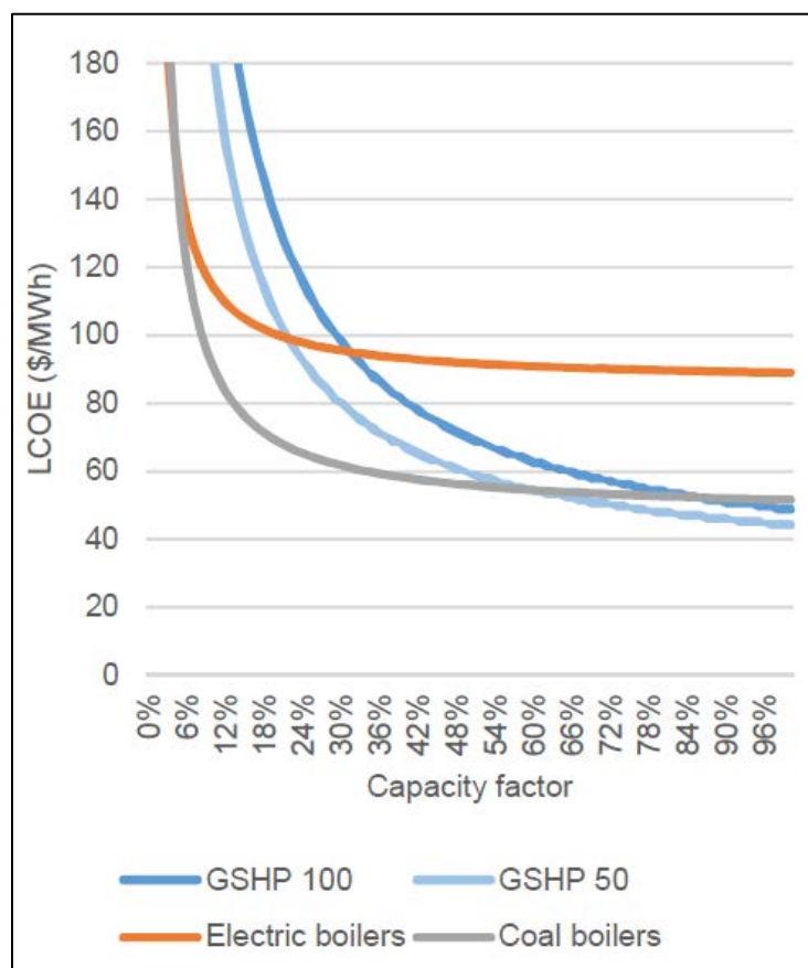
Figure 84: LCoE analysis for various heating technologies.
