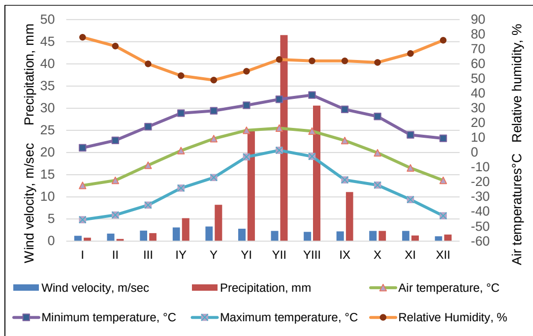
Figure 39: Umnugovi climatogram.
