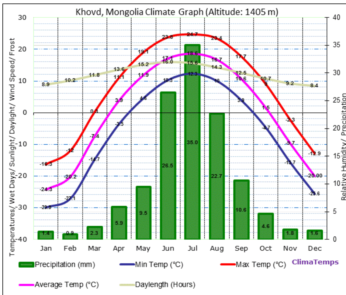
Figure 75: Khovd climatogram.
