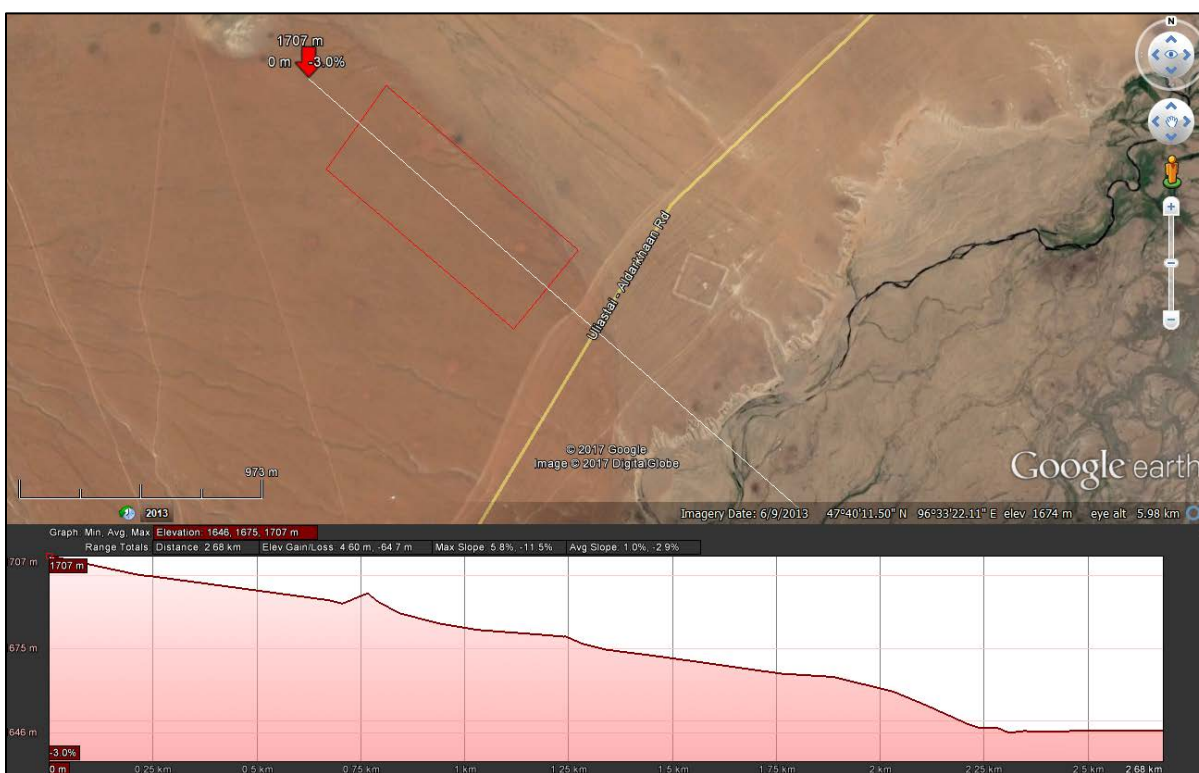
Figure 47: Uliastai Solar PV site topographical profile.
