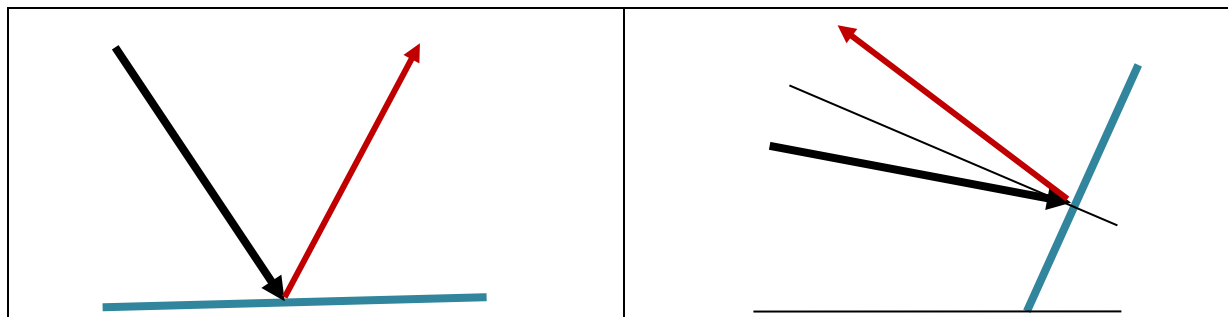
Figure 77: Example of solar glare from horizontal and angled surfaces.
