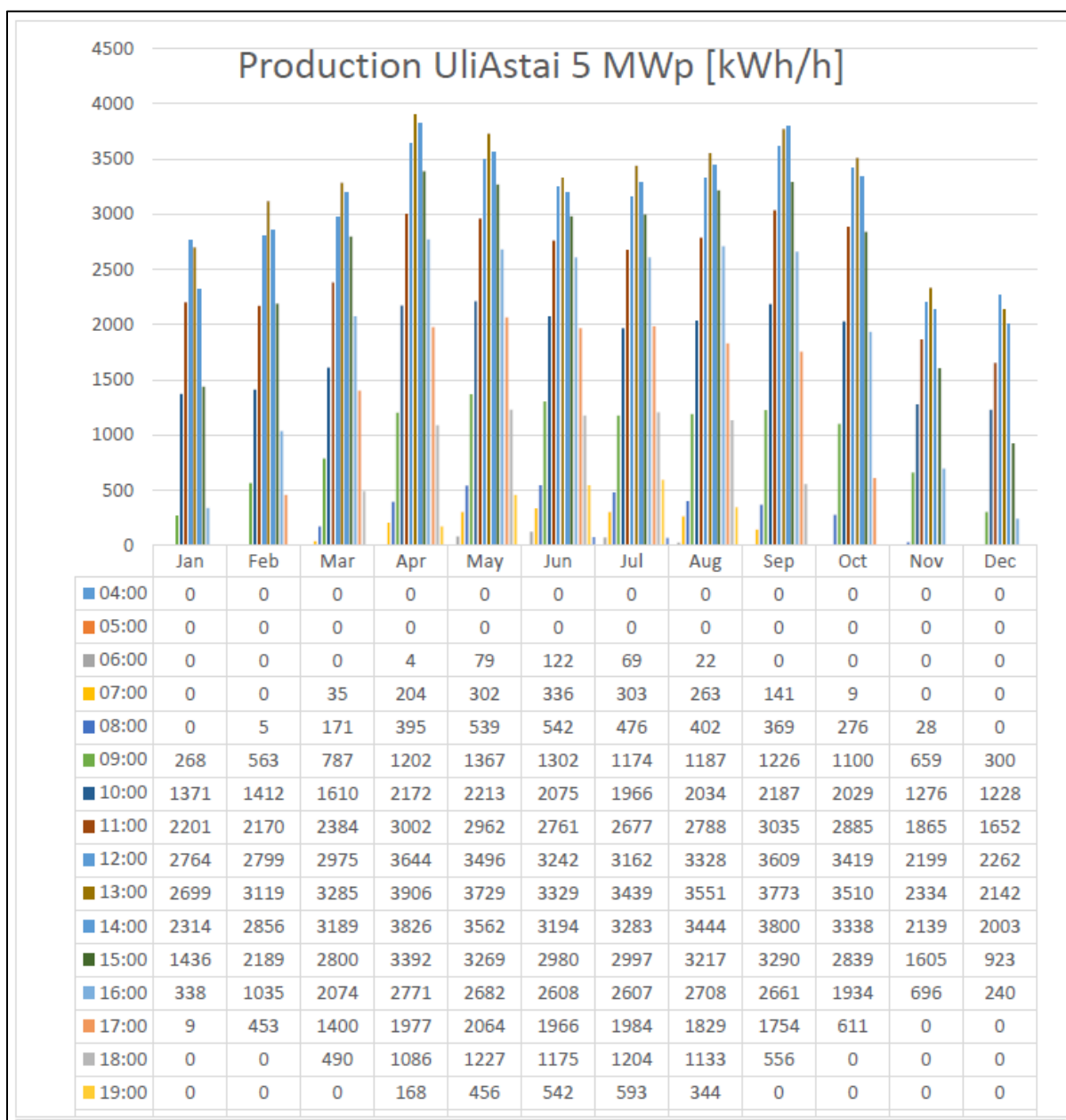
Figure 10: Uliastai solar PV farm estimated production (kWh/hr).
