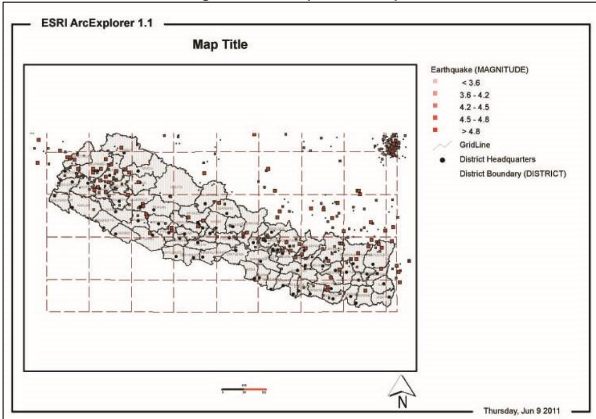
Figure 3a: Earthquakes in Nepal
