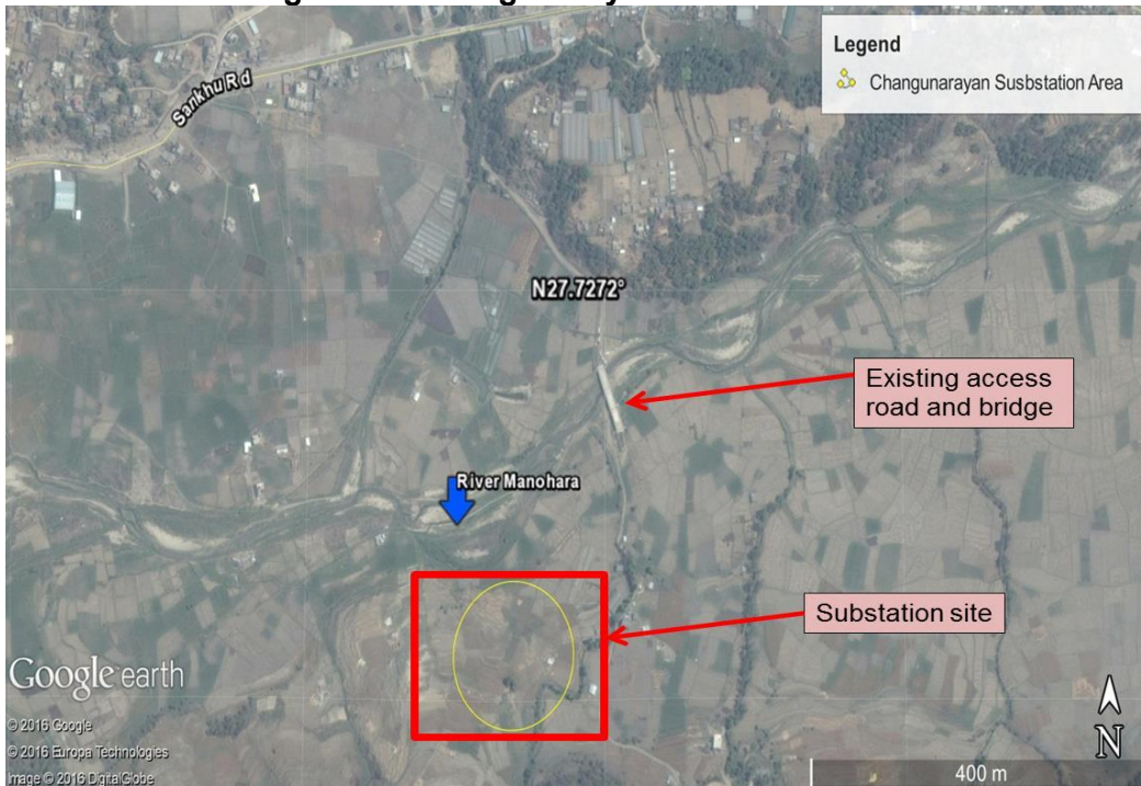
Figure 15: Changunarayan Substation Site
