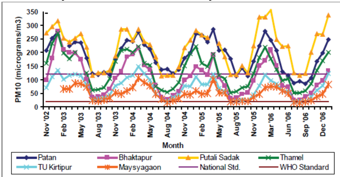
Figure 10: Monthly PM10 Levels in Kathmandu Valley November 2002 – December 2006
