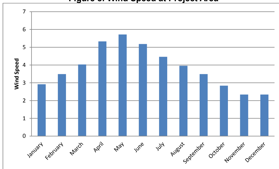
Figure 8: Wind Speed at Project Area
