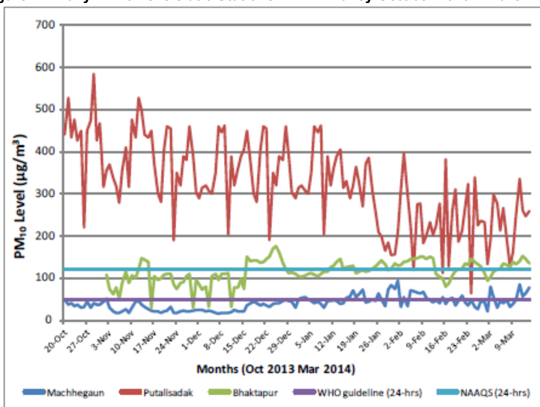
Figure 11: Daily PM10 Levels at 3 Stations in KTM Valley October 2013 – March 2014
