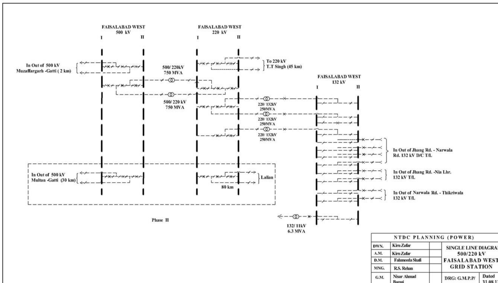
Fig 2.2: Single Line Diagram 500/220 Faisalabad West Grid Station
