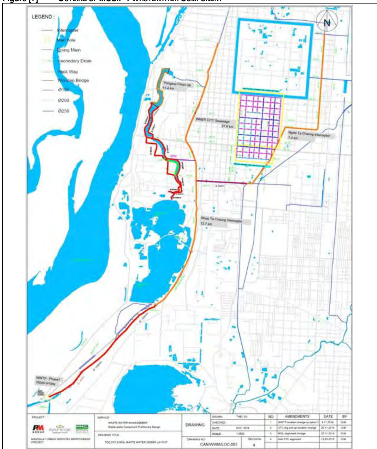
Figure [7] OUTLINE OF MUSIP 1 WASTEWATER COMPONENT
