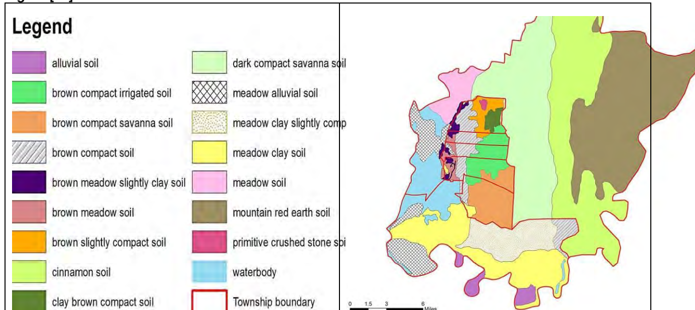
Figure [16] SOIL MAP OF MANDALAY CITY
