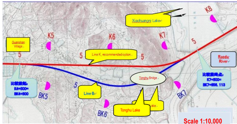
Figure2- 1Comparison of Routing Options for the Tonghu Lake Segment
