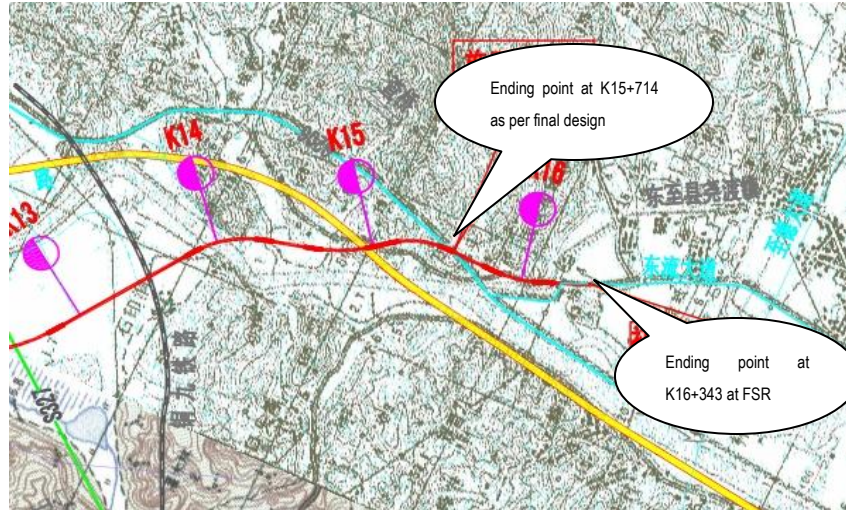
Figure2- 5Comparison of Options G206-Dongliu Road Segment
