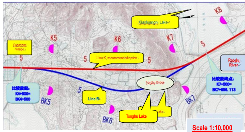
Figure2- 1Comparison of Routing Options for the Tonghu Lake Segment
