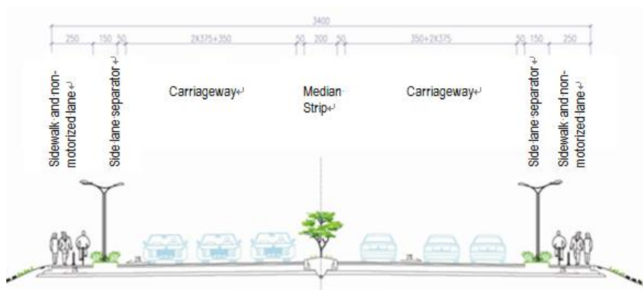
Figure 1-1 Standard Cross-sectional View of the Proposed Highway
