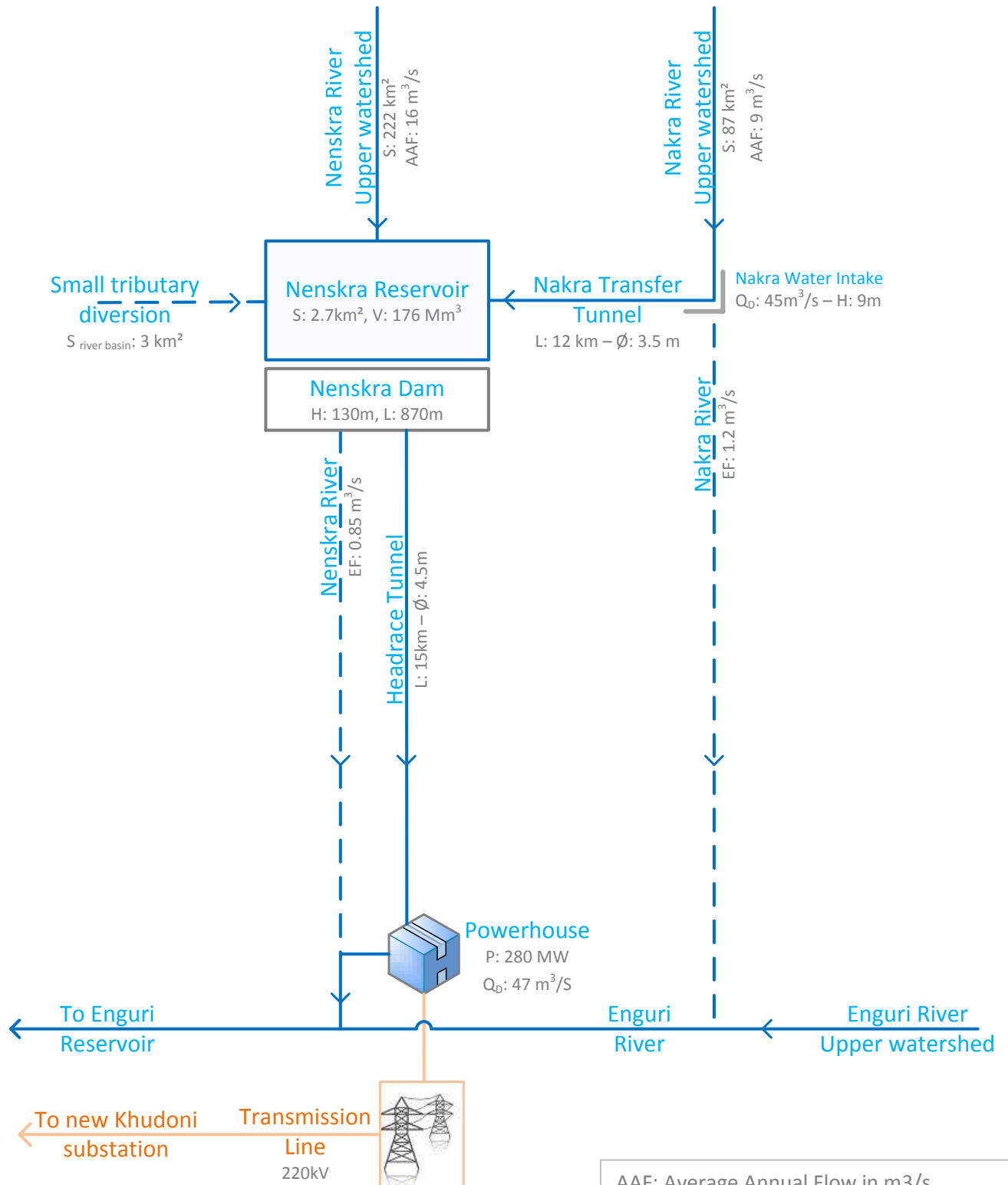
Figure 5 - Nenskra HPP schematic diagram
