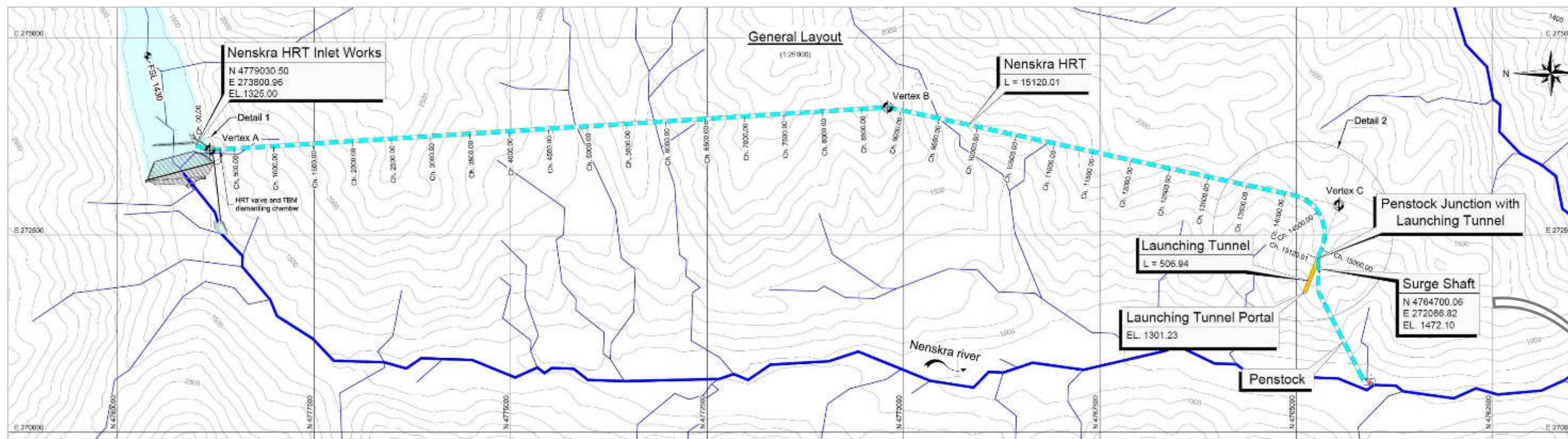
Figure 19 - General layout of the main water way From L-6768-B-UW-HR-GE-DW-001 000
