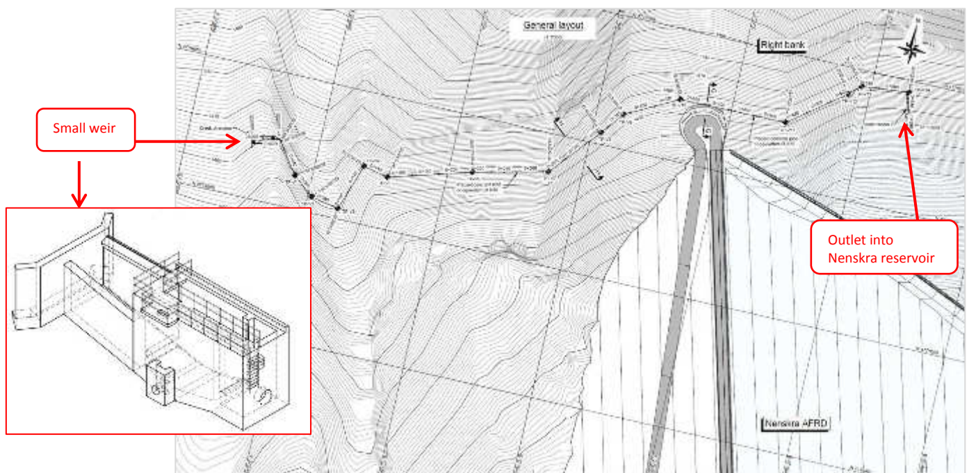
Figure 15 - Small seasonal tributary diversion on the right bank downstream of the dam From L-6768-B-CW-CD-GE-DW-001_000 and L-6768-B-CW-CD-GE-DW-003_000
