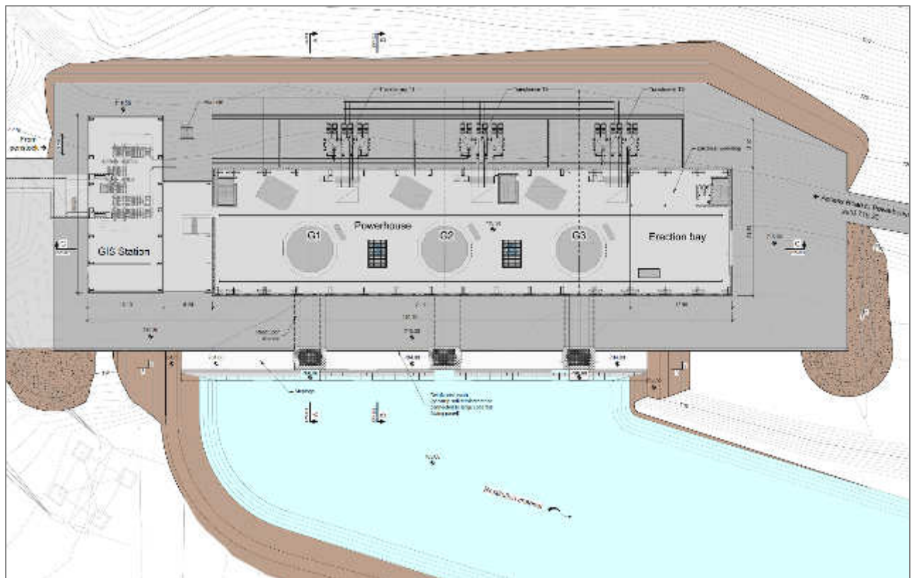
Figure 26 - Powerhouse plan at ground level From L-6768-B-CW-PH-GE-DW-201_001
