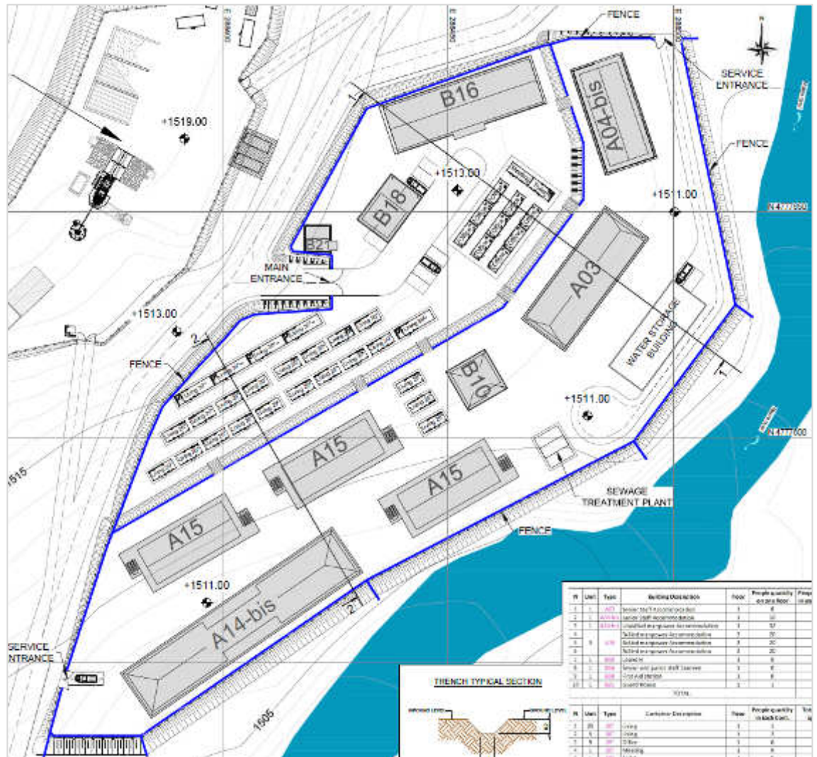
Figure 37 - Layout of the camp at the Nakra intake site
