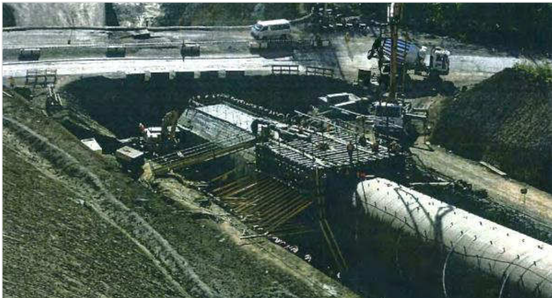
Figure 46 - Illustration of penstock construction stages - Taken from another project. Top right: concrete slab in bottom trench, Top left: installation of the penstock steel liners Bottom: reinforced concrete box over the penstock steel liners Source: Salini Impregilo
