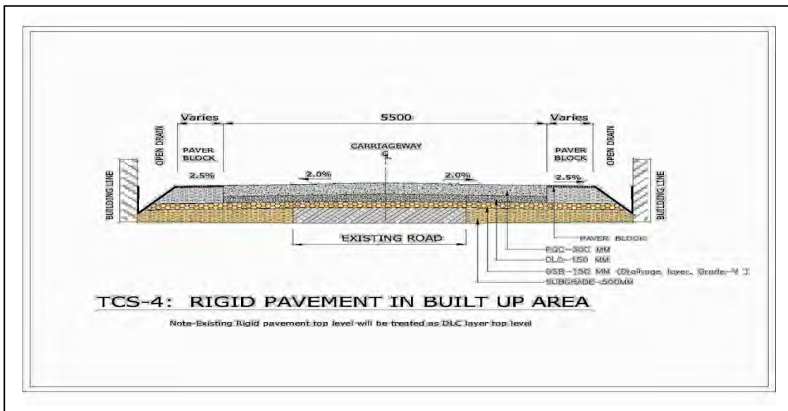
Figure 4: Rigid Pavement in Built Up Area
