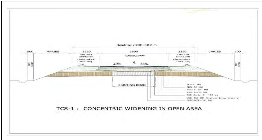
Figure 3: Concentric Widening in Open Area
