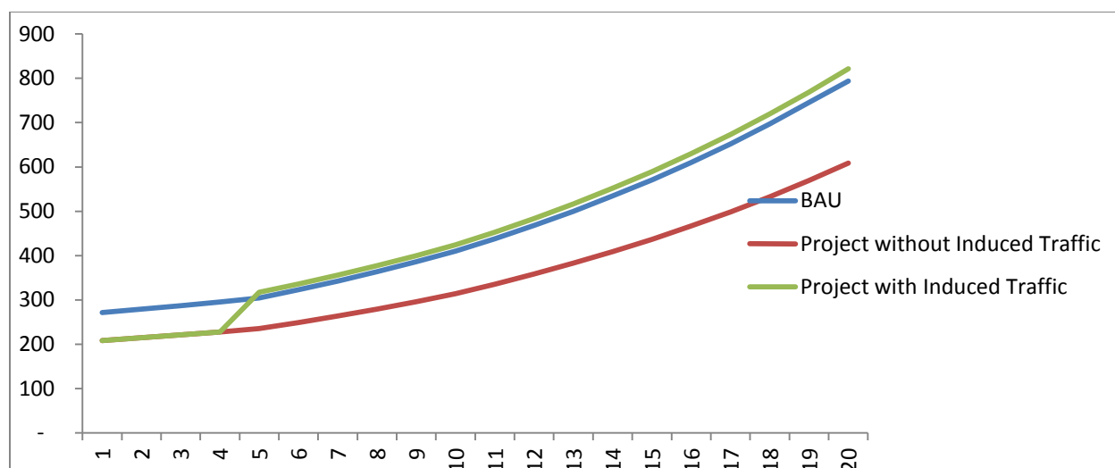
Figure 5.1: Plot of CO 2 Emissions Considering Improvement in Surface Roughness and Road Capacity
