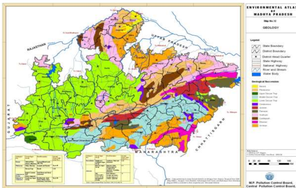
Figure: 4.1: Geological Map of MP
