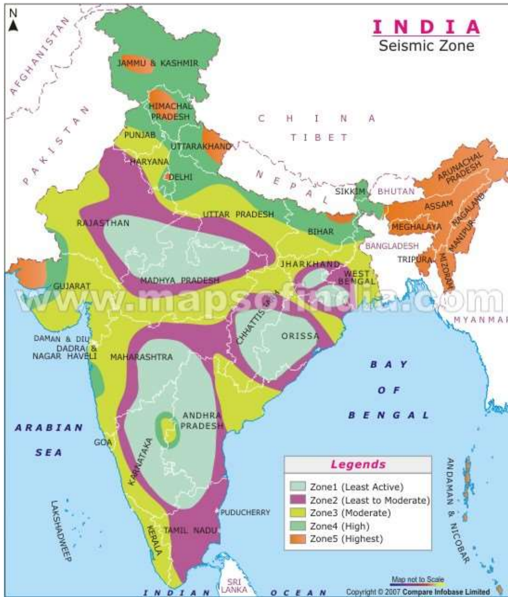
Figure 4.3: Seismic Zone Map of India
