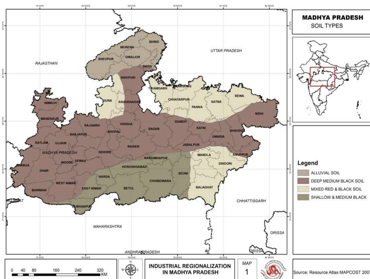
Figure 4.2: Soil Map of MP
