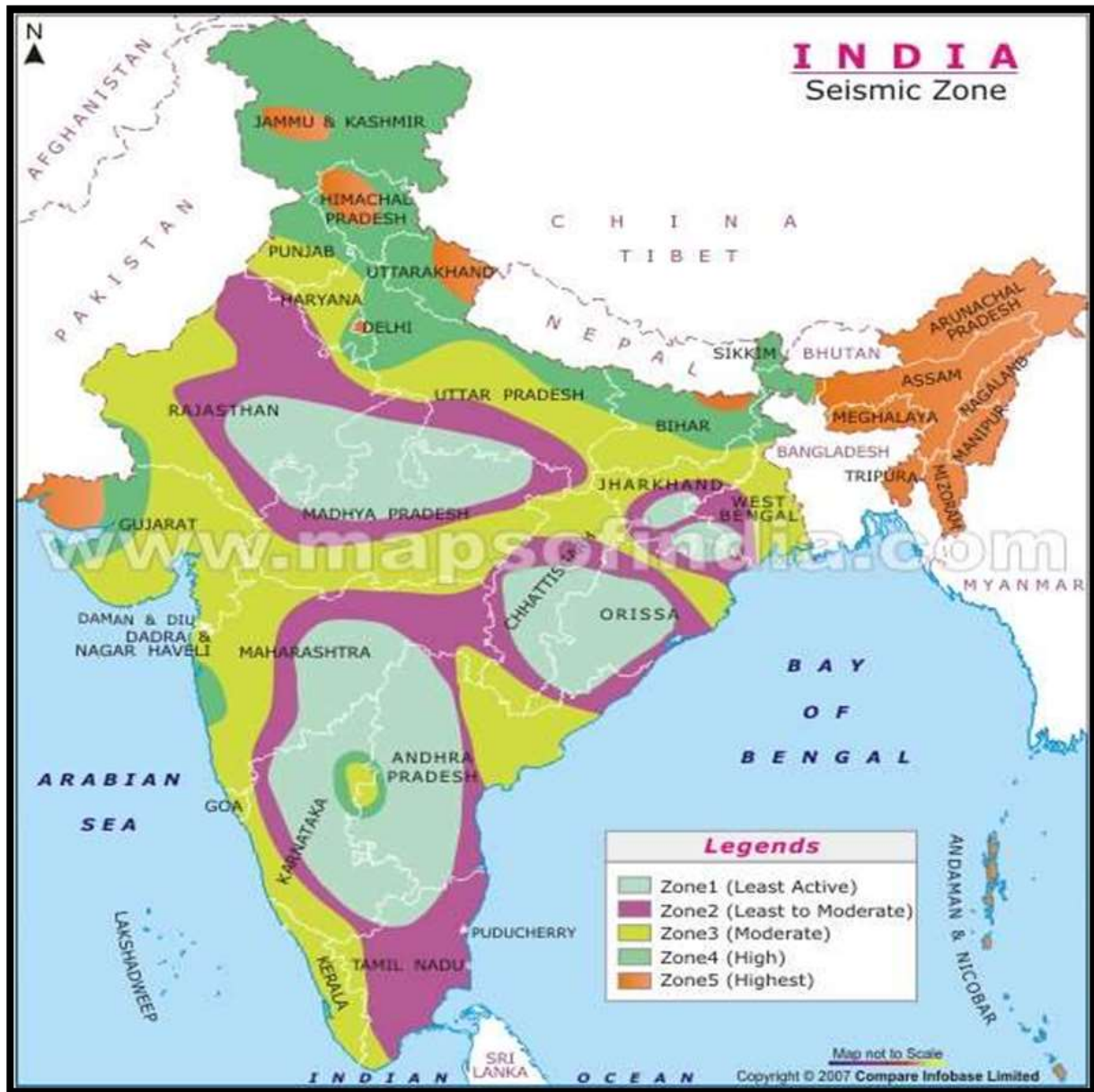
Figure 7: Seismic Zone Map of India
