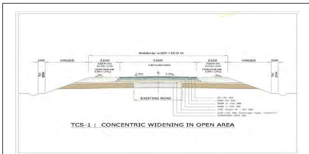
Figure 3: Typical Cross Section of Geometric Realignment
