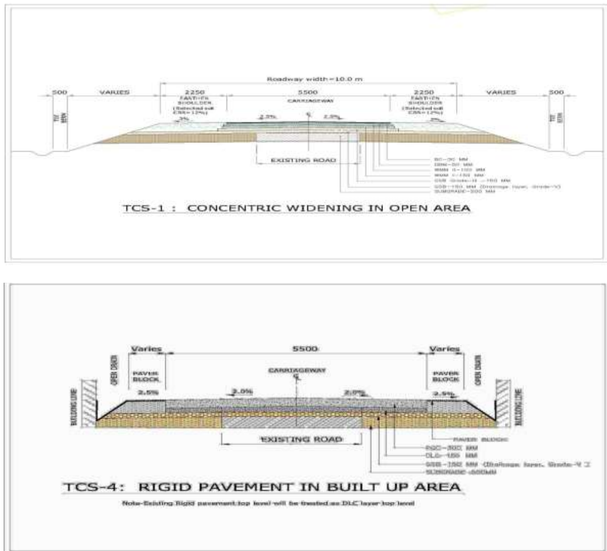
Figure 3 & Figure 4: Typical Cross-section of Geometric Realignment
