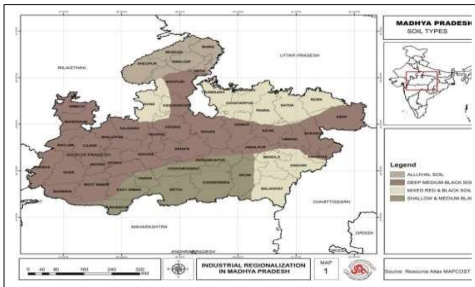
Figure 7: Soil Map of MP
