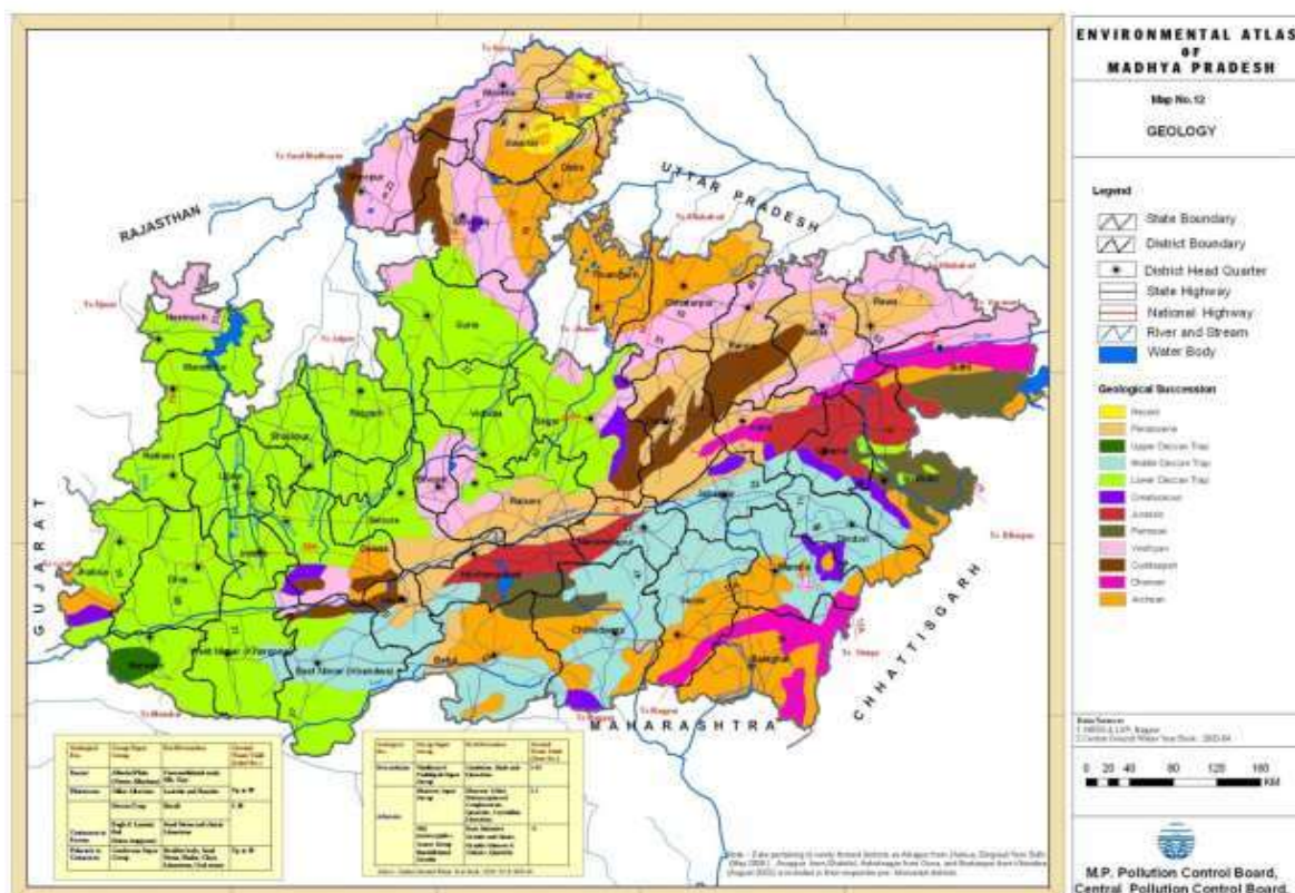
Figure 6: Geological Map of MP
