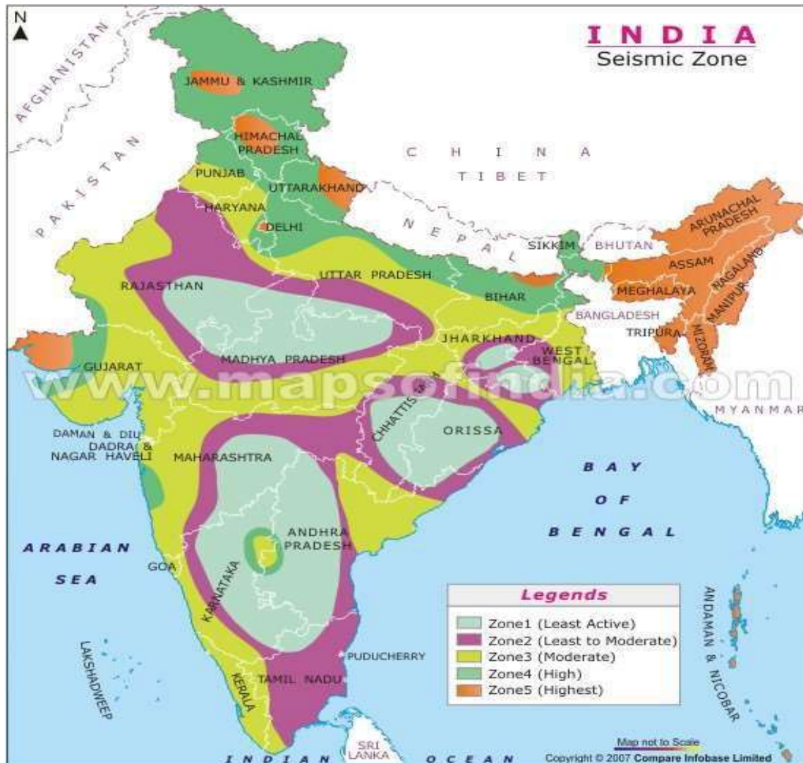
Figure 7: Seismic Zone Map of India
