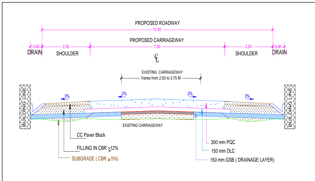
Figure 3: Typical Cross-section of CC Pavement
