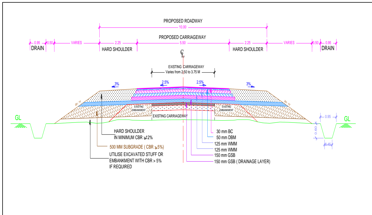
Figure 2: Typical Cross-section of Flexible Pavement
