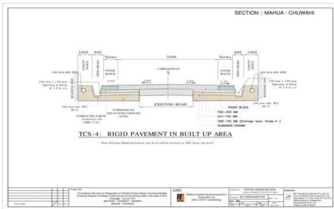
Figure 3.2. Typical Cross-Section in Built-up Areas
