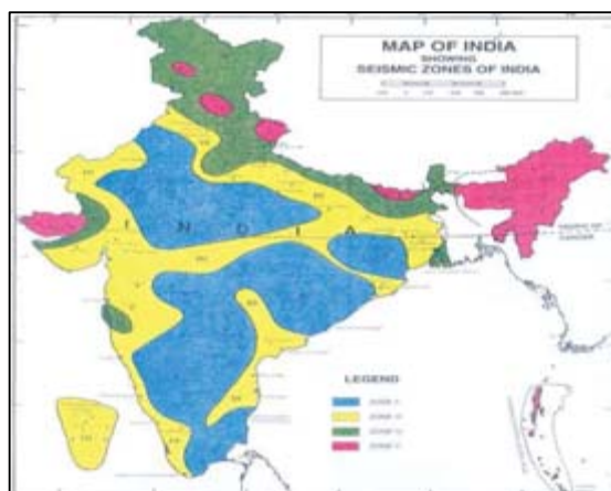
Fig.6. Seismic Zone of India
