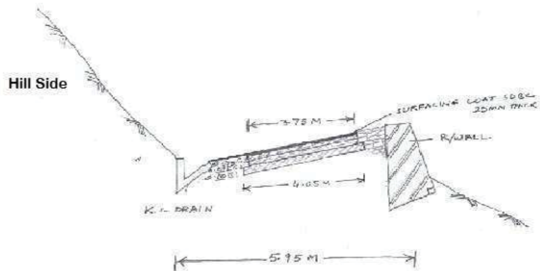
Fig. 3. Typical Road Cross Section
