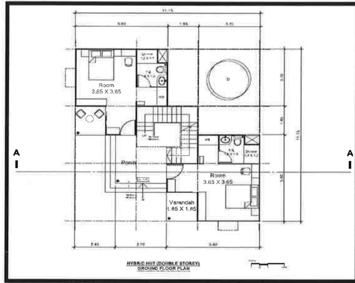
(i) Hybrid Ground Floor Plan
