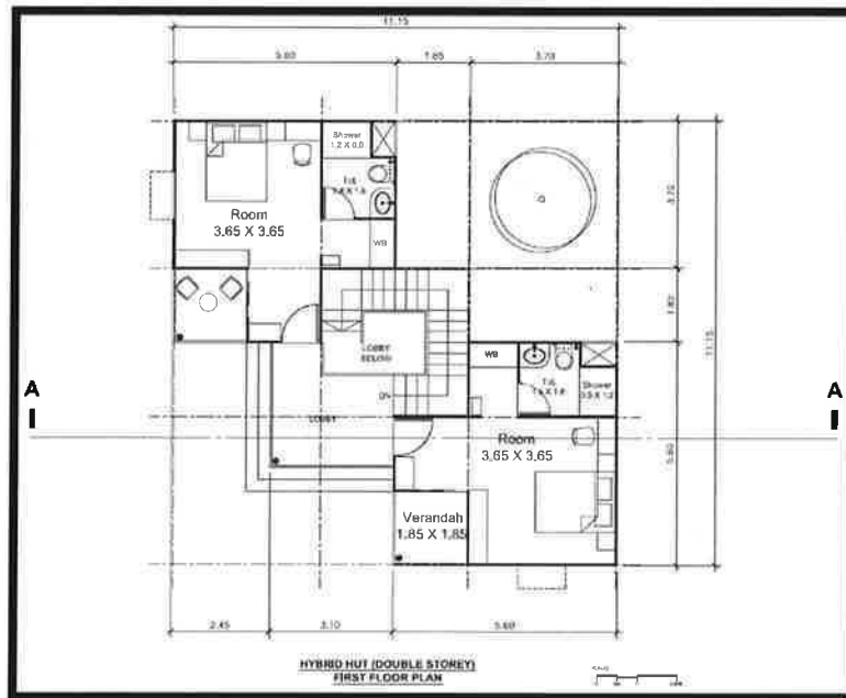
(ii) First Floor Plan
